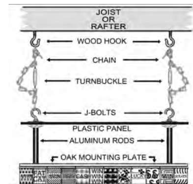
Over-the-Counter Display Tile Mounting
